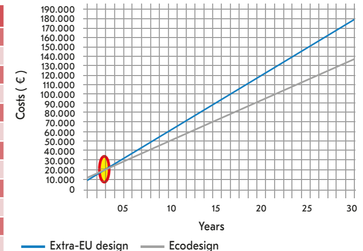
Ecodesign Transformer compared with Extra-EU design
