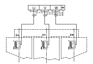
PT 100 ohm Connections Diagram
