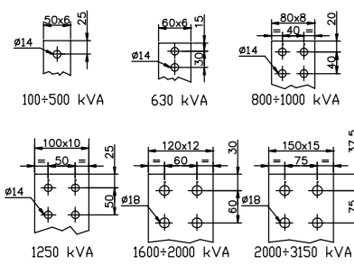
LV Terminal
